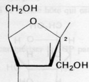
\beta -D-fructofuranose
