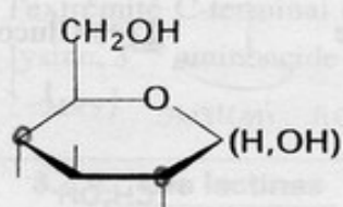
D-glucopyranose
